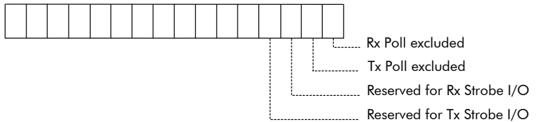
Figure 4-1 Word Bits Set for Exclusion of Polled I/O and Strobed I/O
