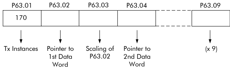
Figure 4-2 I/O Packet Word Structure
