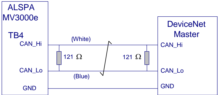
Figure 3-1 Network Cabling between an ALSPA MV3000e Drive and a DeviceNet Master
