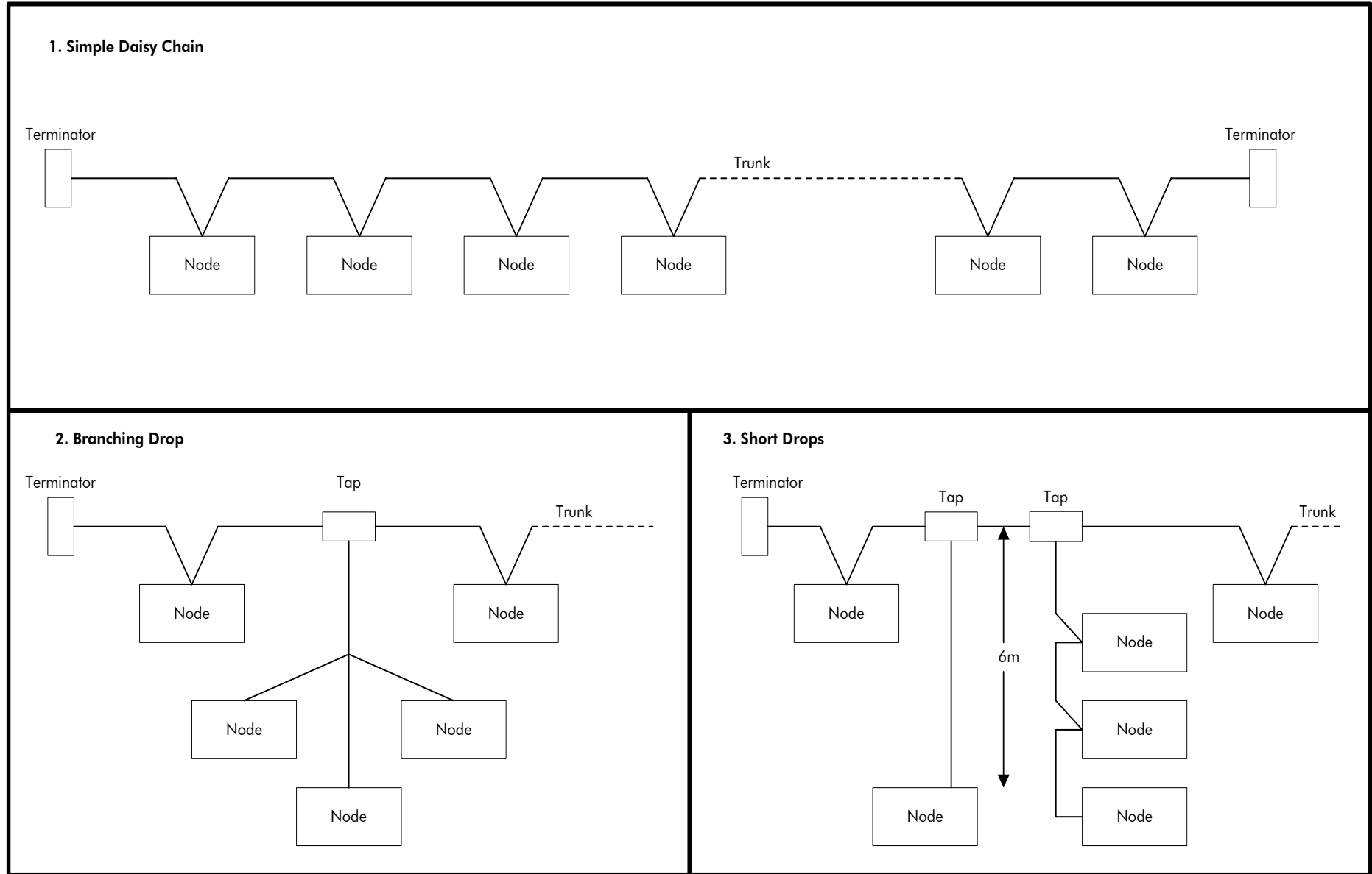
Figure 1. Network Topologies
