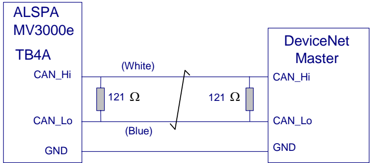
Figure 3-2 Network Cabling between an ALSPA MV3000e Drive and a DeviceNet master.
