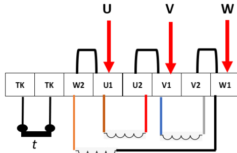
Alternative Connection – Delta Mode
