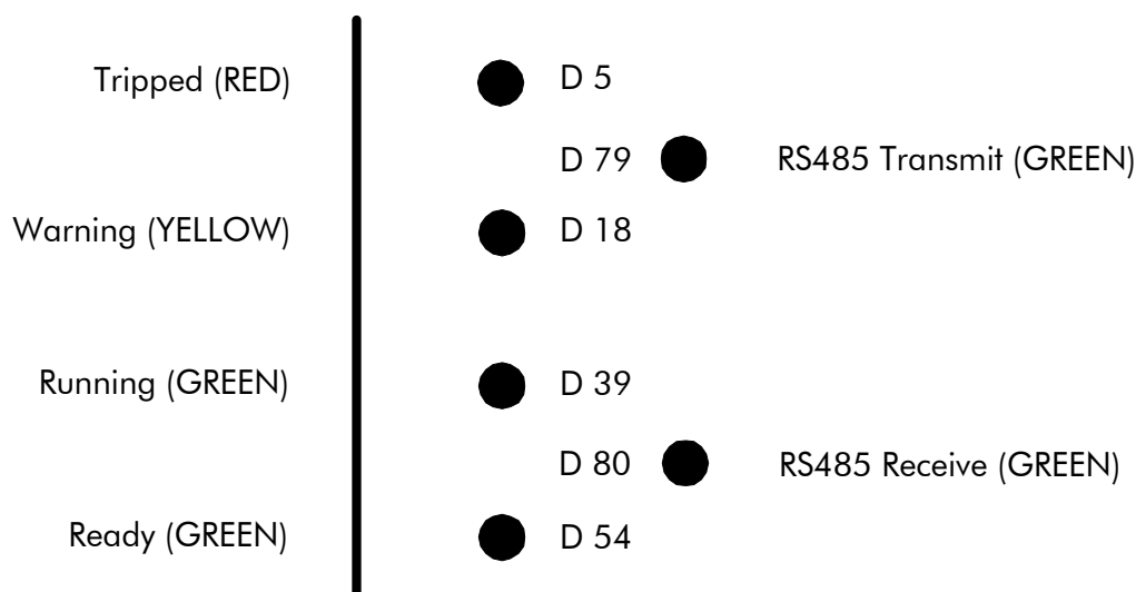
Figure 8-2 Functions of LEDs for MV3000e Controller for DELTA Modules
