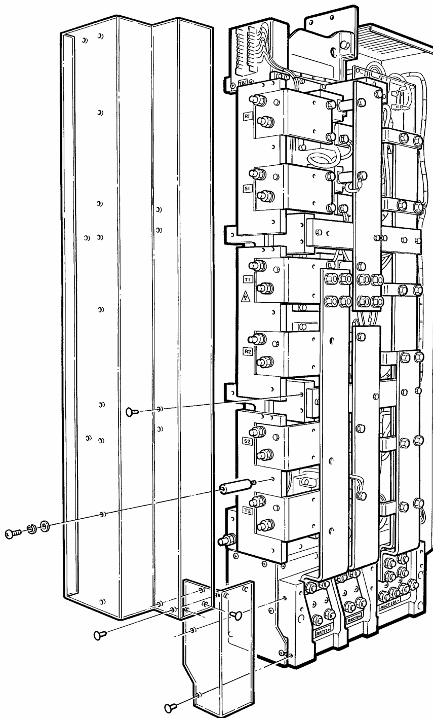
Figure 6-3 Rectifier Bridge Module Shrouds
