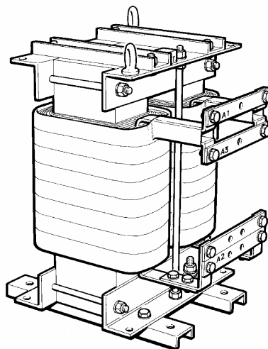
Figure 1-12 Interbridge Transformer 50Z0119/02 for 12 Pulse Rectifier Systems
