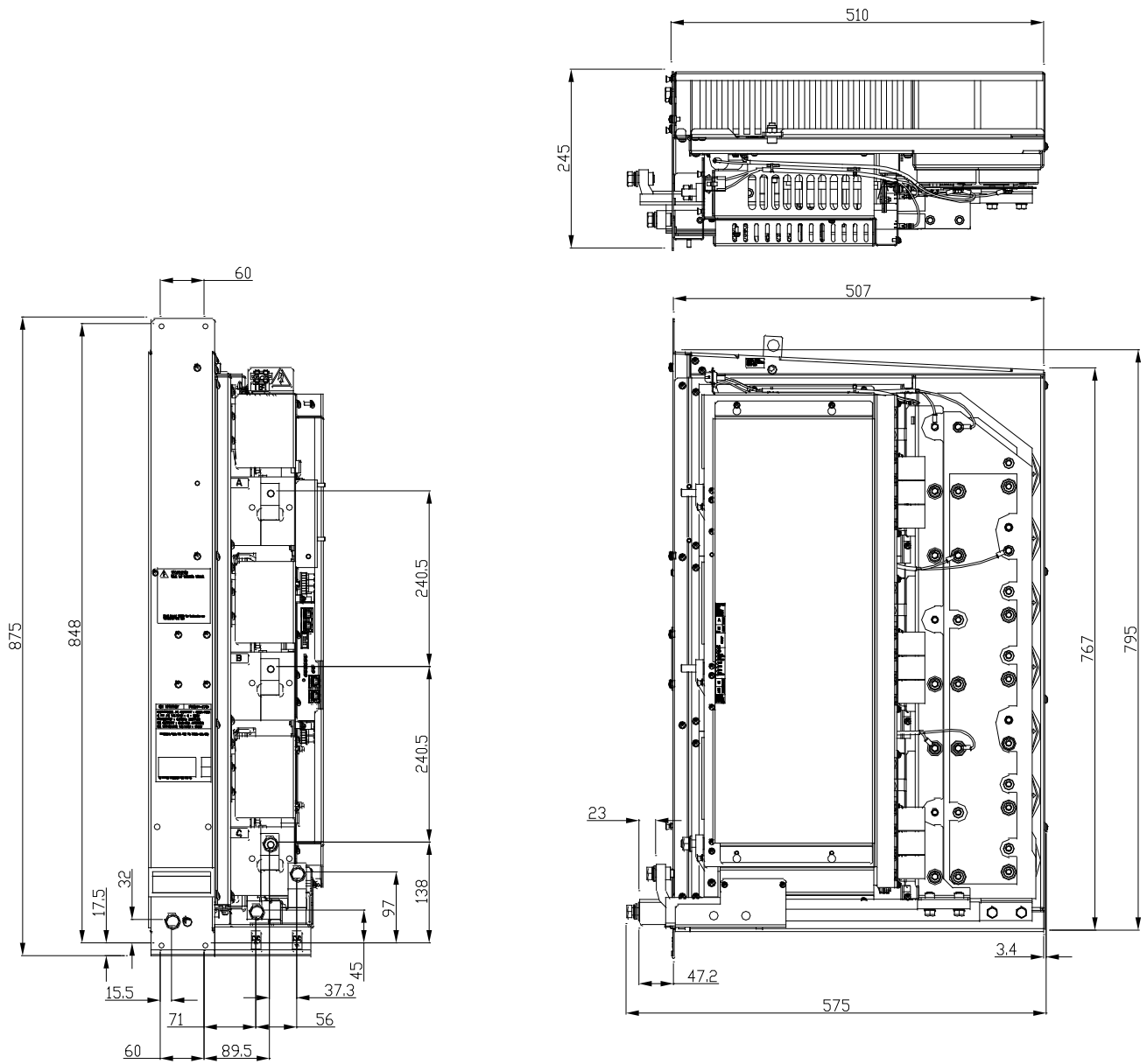
Figure 3-1. – PED500 Dimensions (shrouds not shown)
