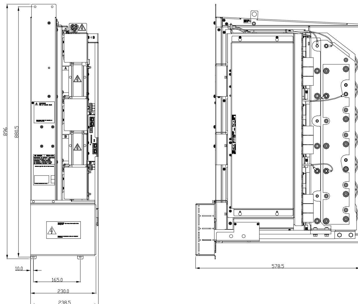
Figure 3-2. – PED500 Dimensions including shrouds
