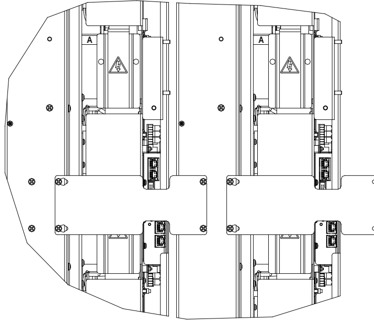
Figure 4-1. – Bonding plate linking adjacent DELTAs
