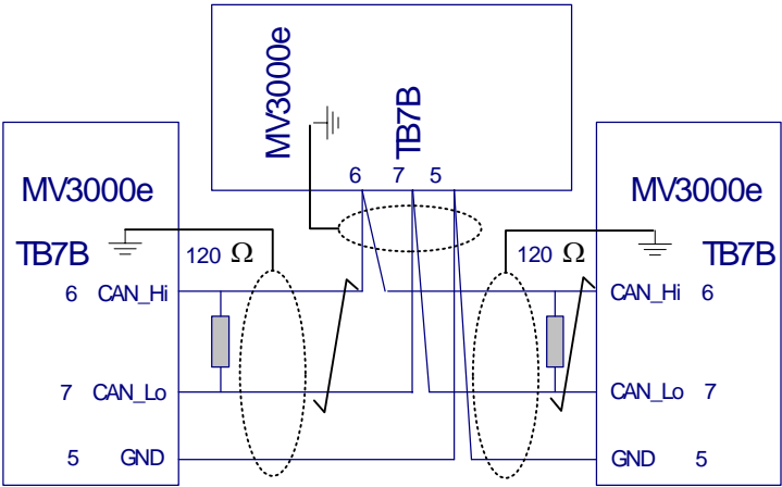
Figure 4-2. – Network Cabling between 3 Nodes
