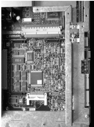
Figure 3-7. – DELTA System – positioning the CAN2 Board
