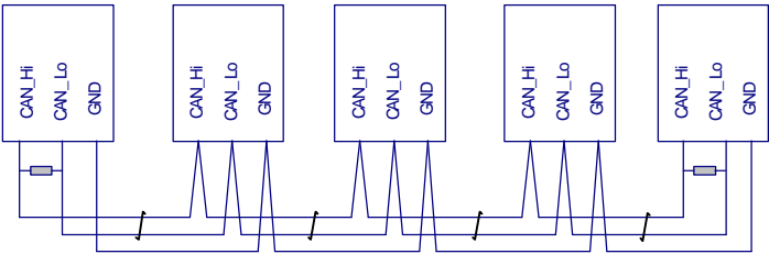
Figure 4-3. – Network Cabling between more than 3 Nodes
