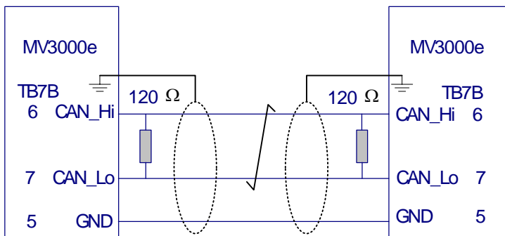
Figure 4-1. – Network Cabling between 2 Nodes
