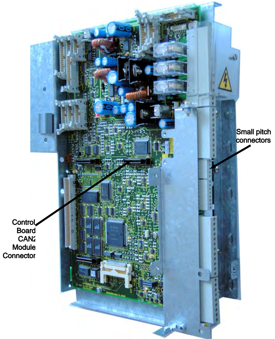
Figure 3-3. – Location of CAN2 connector & small pitch connectors
