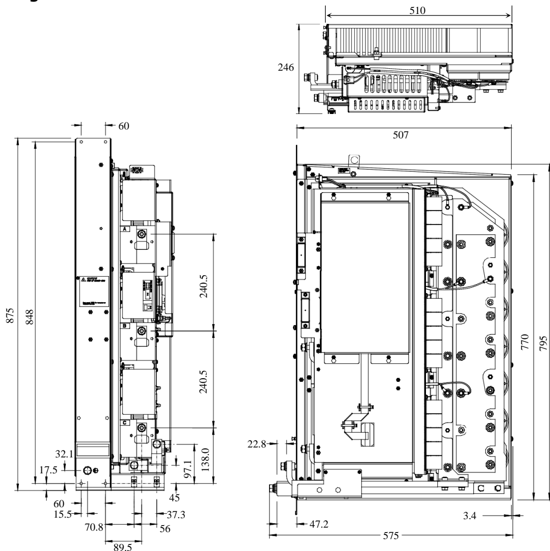
Figure 5.1 – Dimensions without shrouds
