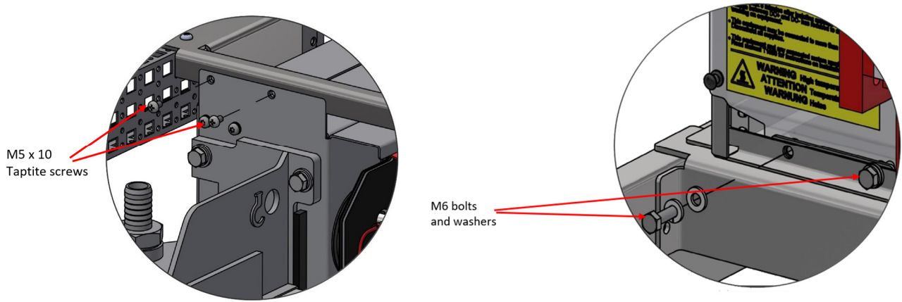
Figure 11-11. Securing fasteners (top and bottom)
